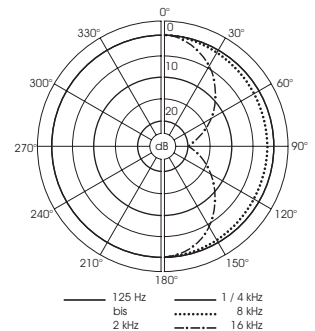
Polar patterns
