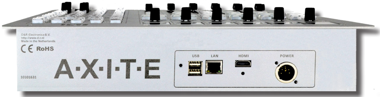
Backpanel Axite main frame with connectors for Power, Flatscreen monitor, Ethernet and USB (future options)
