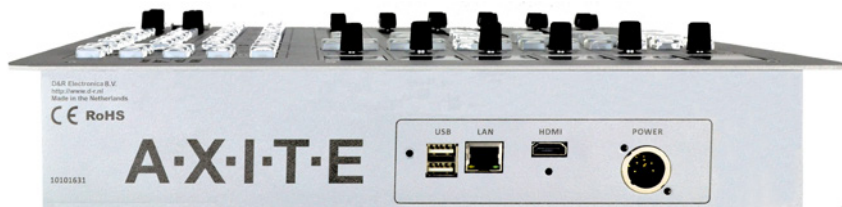
Back panel 6 fader Axite main unit
